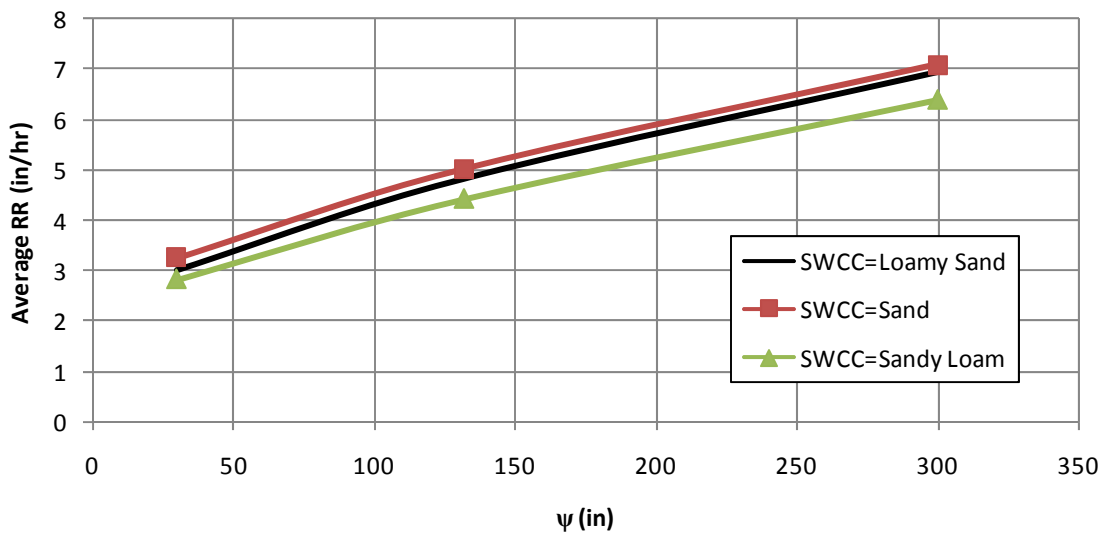
Figure 5.4 Average recession rate (RR) vs. matric suction ( \psi ) for Loamy Sand with SWCC varied.
