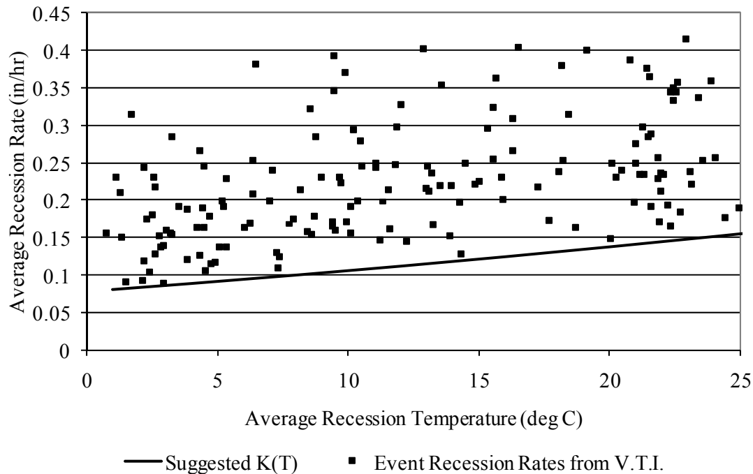
Figure 4.2 Plot of average event recession rates from the Villanova Traffic Island from 2003-2007.
