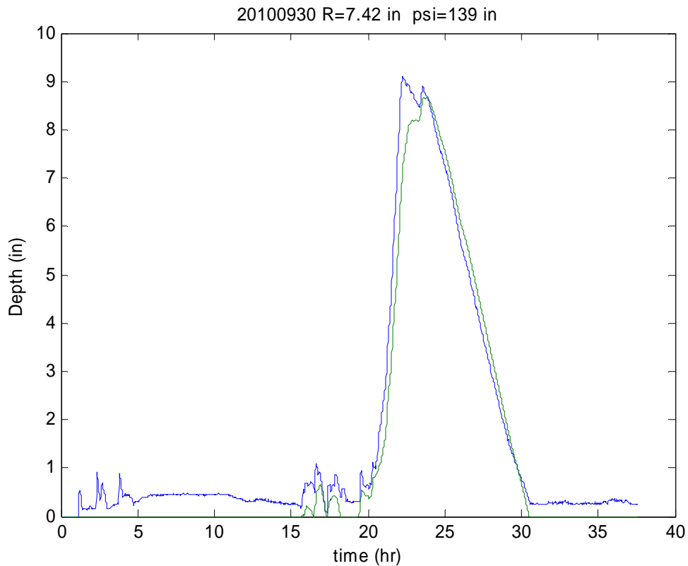
Figure 6.12 Depth vs. time plot from a 7.42 inch rainfall event.
