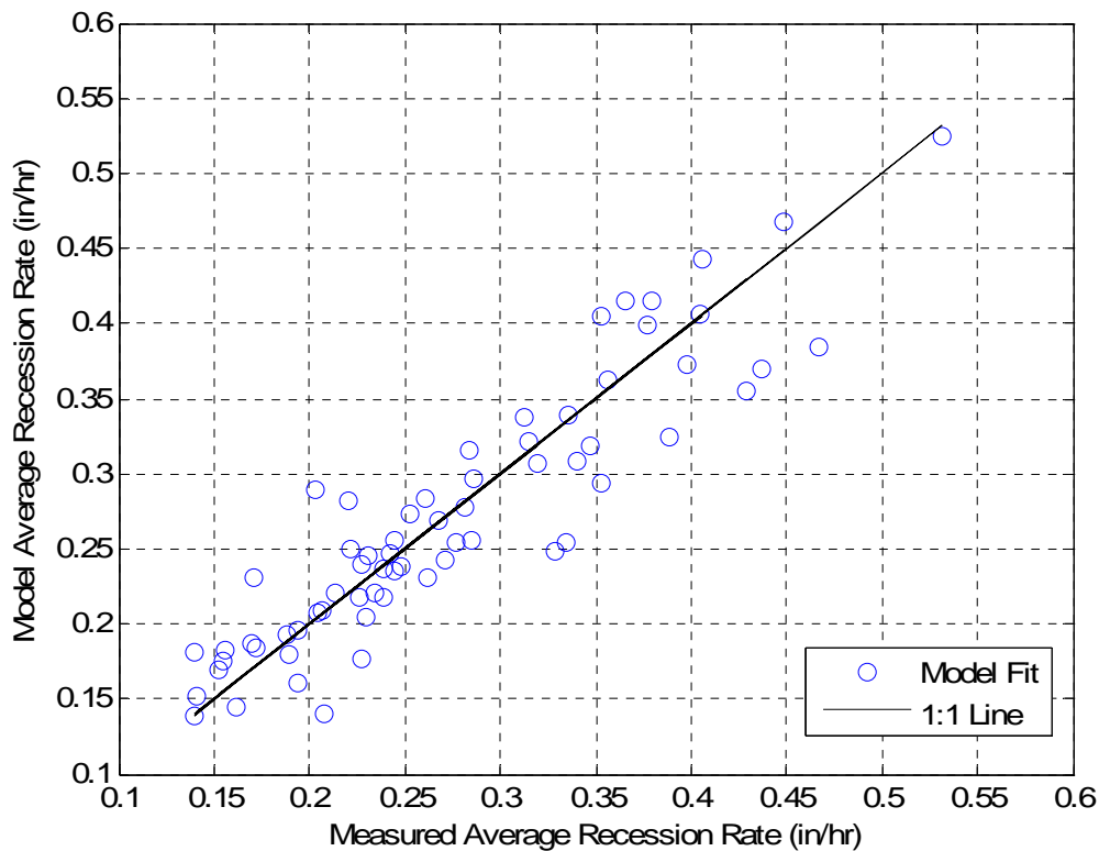
Figure 6.4 Comparison of average recession rates between best-fit model and data.
