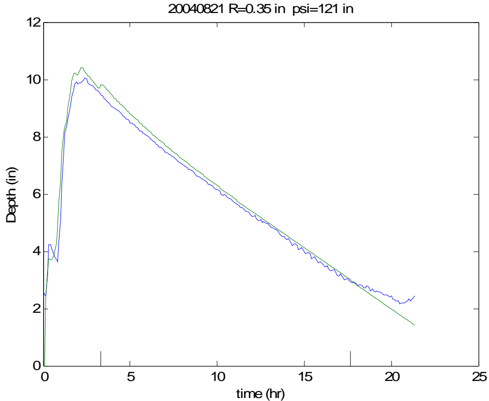
Figure 6.3 Model and Actual depth vs. time for a 0.35 inch rain event. Decreasing infiltration rate is visible.
