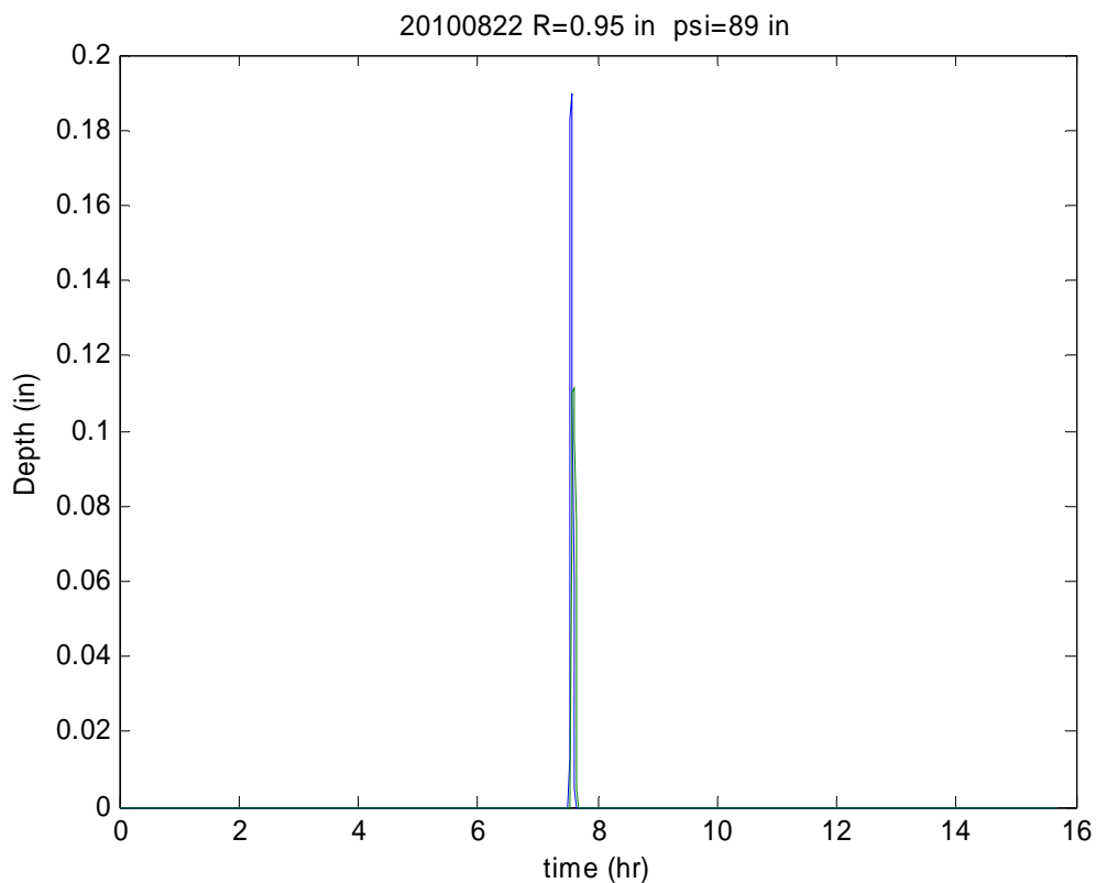
Figure 6.10 Depth vs. time plot from a 0.95 inch rainfall event. Only a brief surge in ponding.
