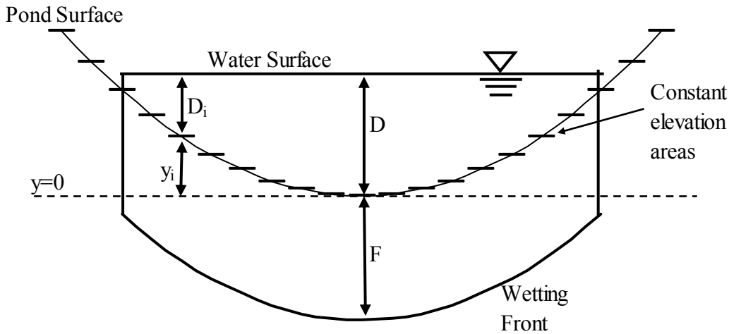
Figure 4.1 Discretization of infiltration bowl geometry.
