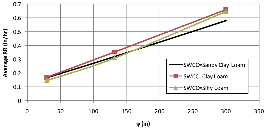
Figure 5.5 Average recession rate (RR) vs. matric suction ( \psi ) for Sandy Clay Loam with SWCC varied.
