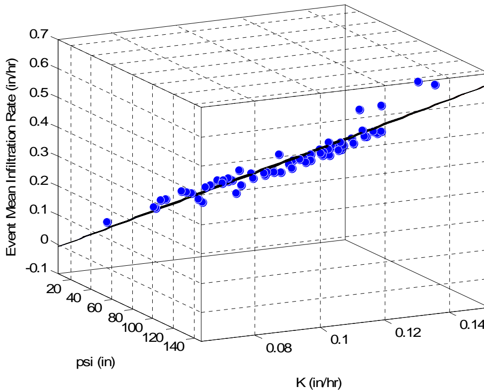
Figure 6.7 Plot of linear regression of mean infiltration rate as a function of K and \psi only. The black line is the cross-section of the plane of best-fit.
