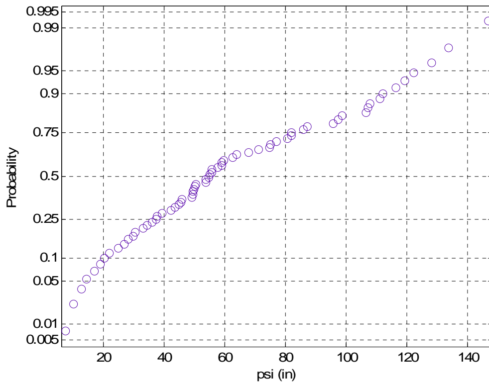
Figure 6.5 Distribution of matric suction values from model correlations.
