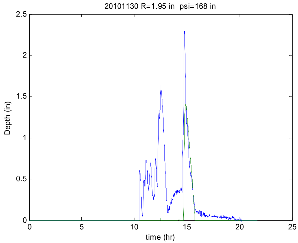
Figure 6.11 Depth vs. time plot from a 1.95 inch rainfall event.
