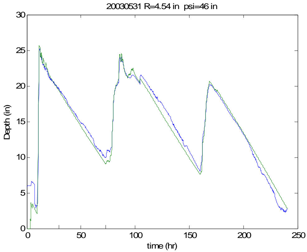
Figure 6.2 Model and actual depth vs. time for a 4.54 inch rain event. Constant infiltration rate is visible.
