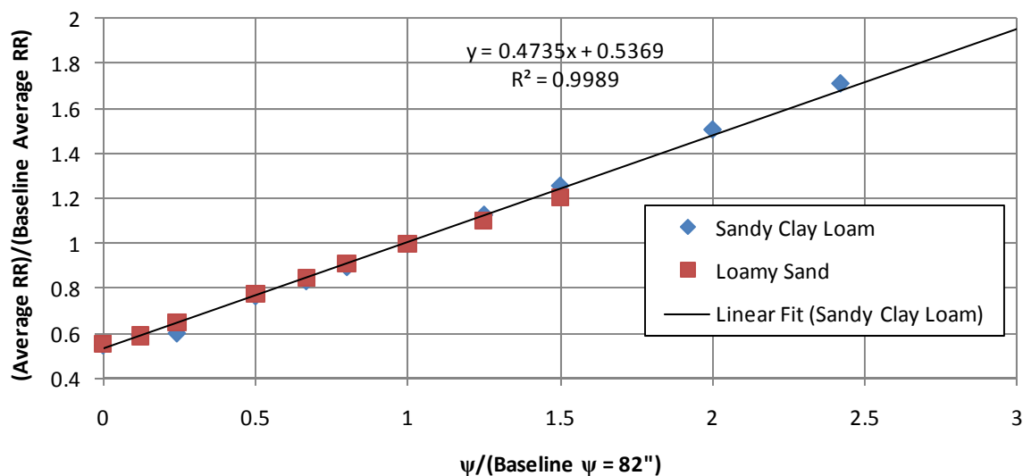
Figure 5.2 Plot of changes in matric suction ( \psi ) vs. change in average recession rate (RR), centered at values of \psi near field capacity (82 inches is center).
