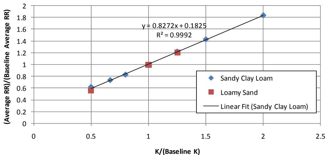
Figure 5.1 Plot of change in conductivity (K) vs. change in average recession rate (RR).
