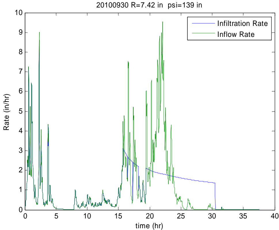
Figure 6.13 Inflow and infiltration rates during the 7.42 inch rainfall event. The rates are equal while the inflow rate is below the infiltration capacity, and so there is no ponding. When the infiltration capacity decreases enough, ponding begins.
