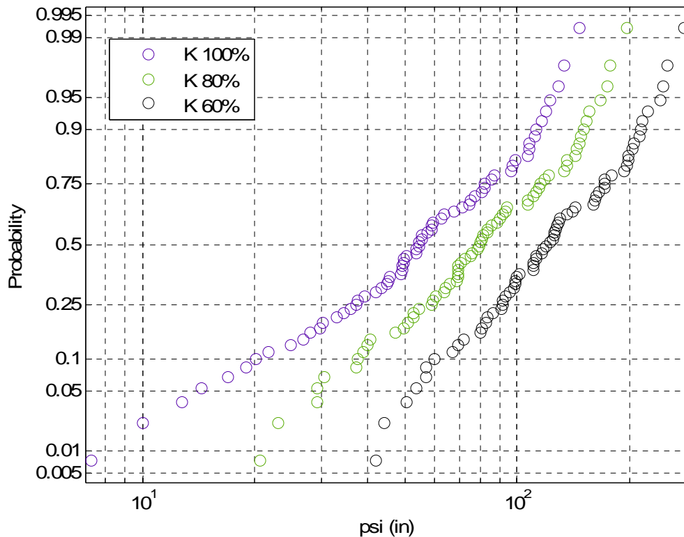
Figure 6.8 Distribution of matric suction values after reducing the conductivity by 20% and 40%.
