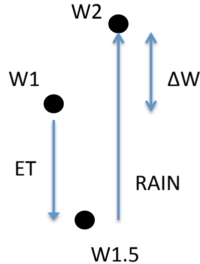
Figure 3.1.4: Demonstration how the change in weight ( \Delta W ) recorded over one day can mislead conclusions about ET. If ET is calculated simply as the change in weight from midnight (W1) to midnight (W2), ET would be considered 0 for the day because the rain (more than) compensates the weight loss due to ET. In this case, ET is the difference between W1 and the lowest weight of day 1 (W1.5). This is equivalent to rain ( P ) minus change in weight from midnight to midnight ( \Delta W ) (Eqn 3.1.2)
